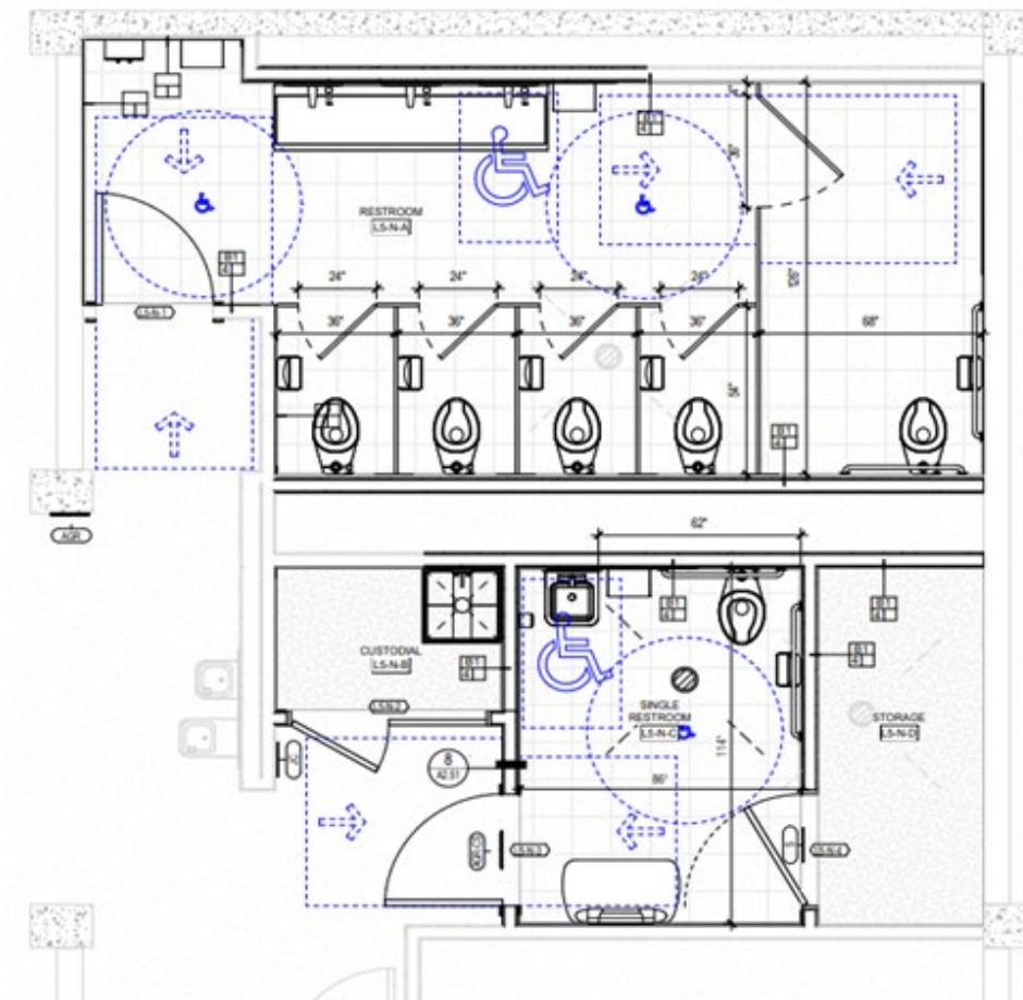
Design Plans
